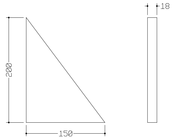
Stiffeners (8 pcs)
